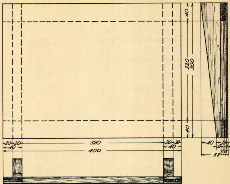
TABL. XXXIV Stolnica
