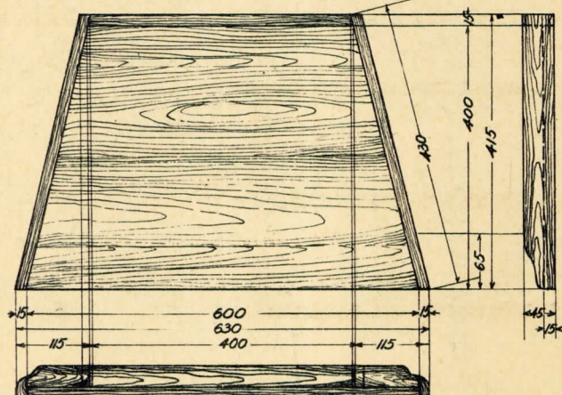
TABL. XXXIV Stolnica
