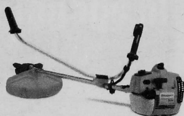
husqvarna 323R 24.5 cm 3 - 0.9 kW / 1.2 KM - 4.5 kg
