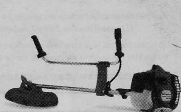
husqvarna 333R 34.6 cm 3 - 1.6 kW / 2.2 KM - 6.1 kg
